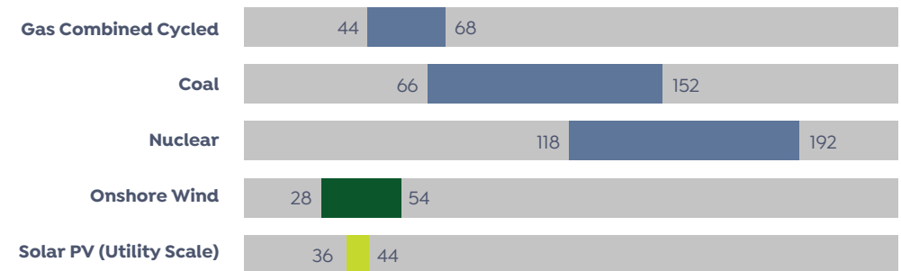
LCOE 3 – By Technology ($/MWh)
